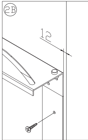
M3,5x16 SV/4
