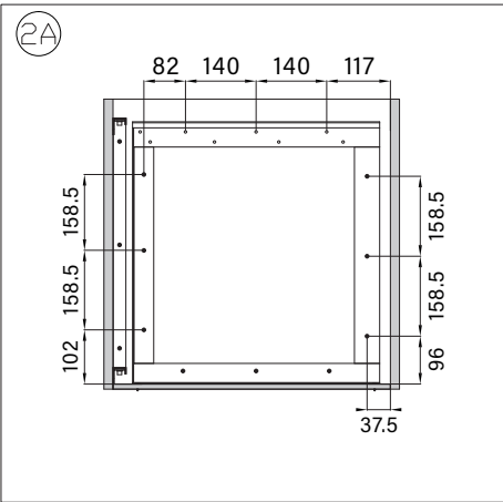
M3,5x16 SV/6
