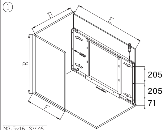
M3,5x16 SV/6
